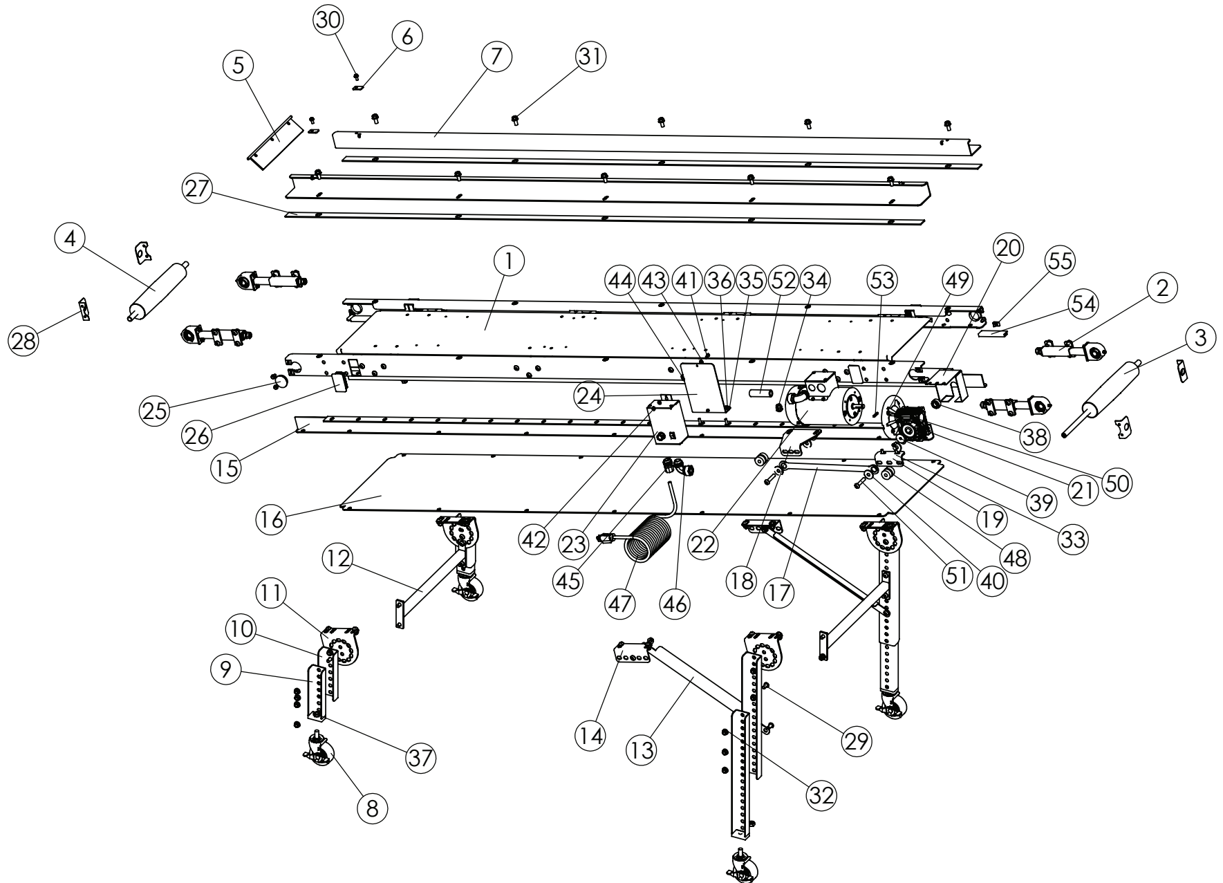
ATLC CONVEYOR - EXPLODED VIEW
