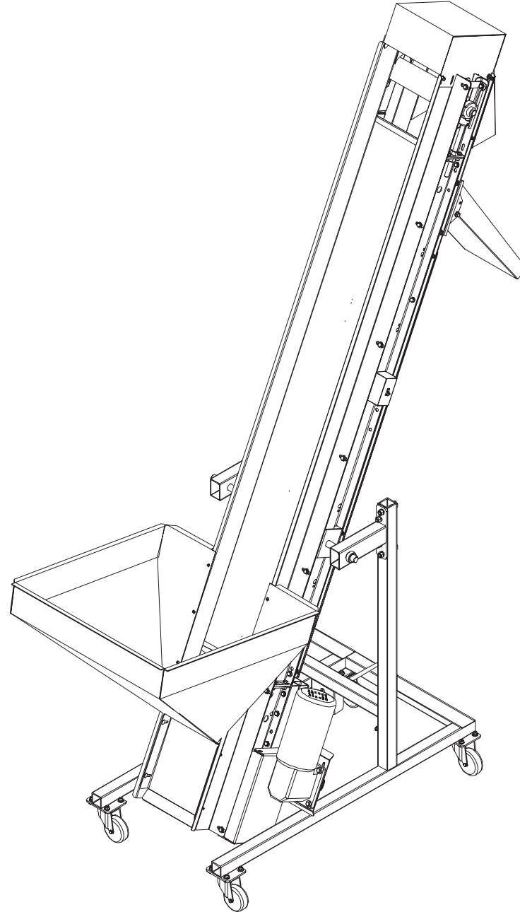
RMSC CONVEYOR - ASSEMBLED VIEW
