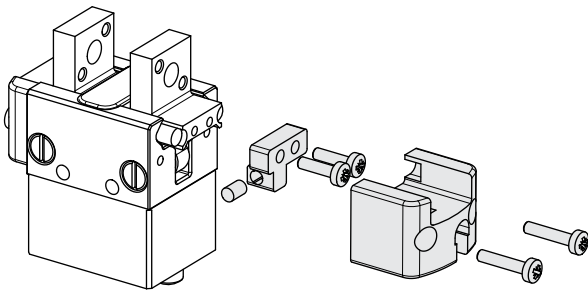
PRO-SN Version
