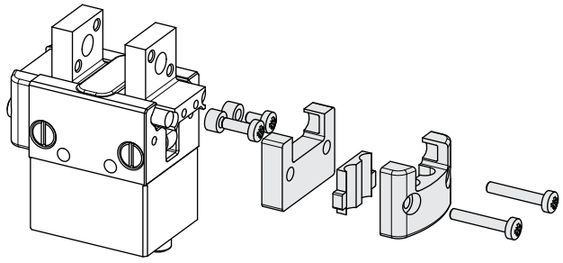
Inductive Version
