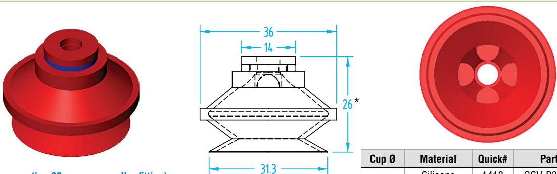
(1st generation 30mm cup—smaller fitting)
