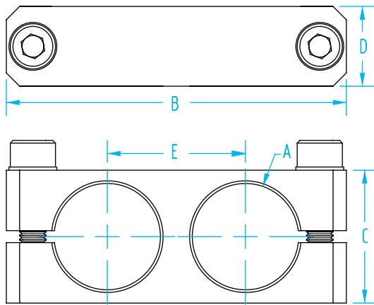
Parallel Clamp
