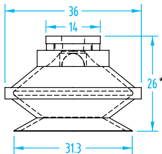
(1st generation 30mm cup—smaller fitting)
