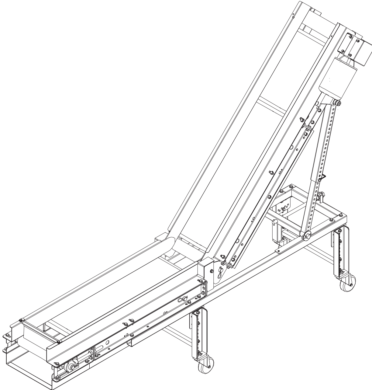
KKI CONVEYOR - ASSEMBLED VIEW
