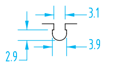
C-Slot dimensional drawing
