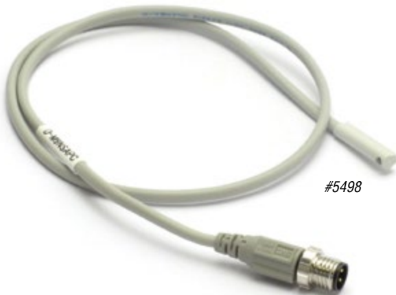
3-Wire Sensors for SMC Cylinders
